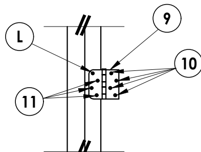
HINGE DETAIL
